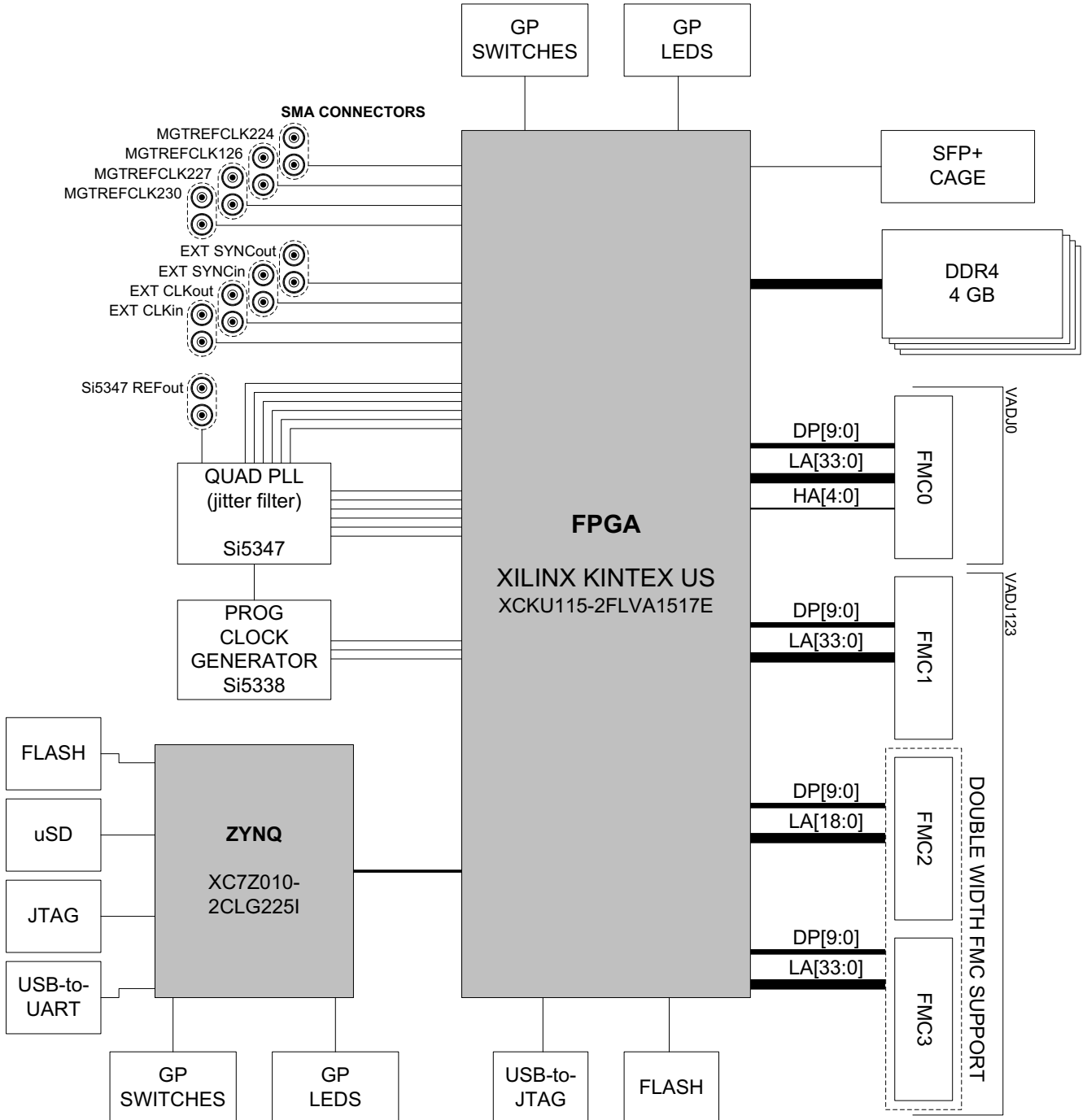
Figure 1: Block Diagram
